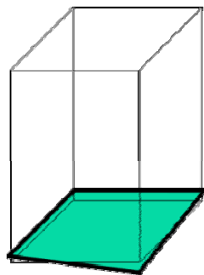
char
